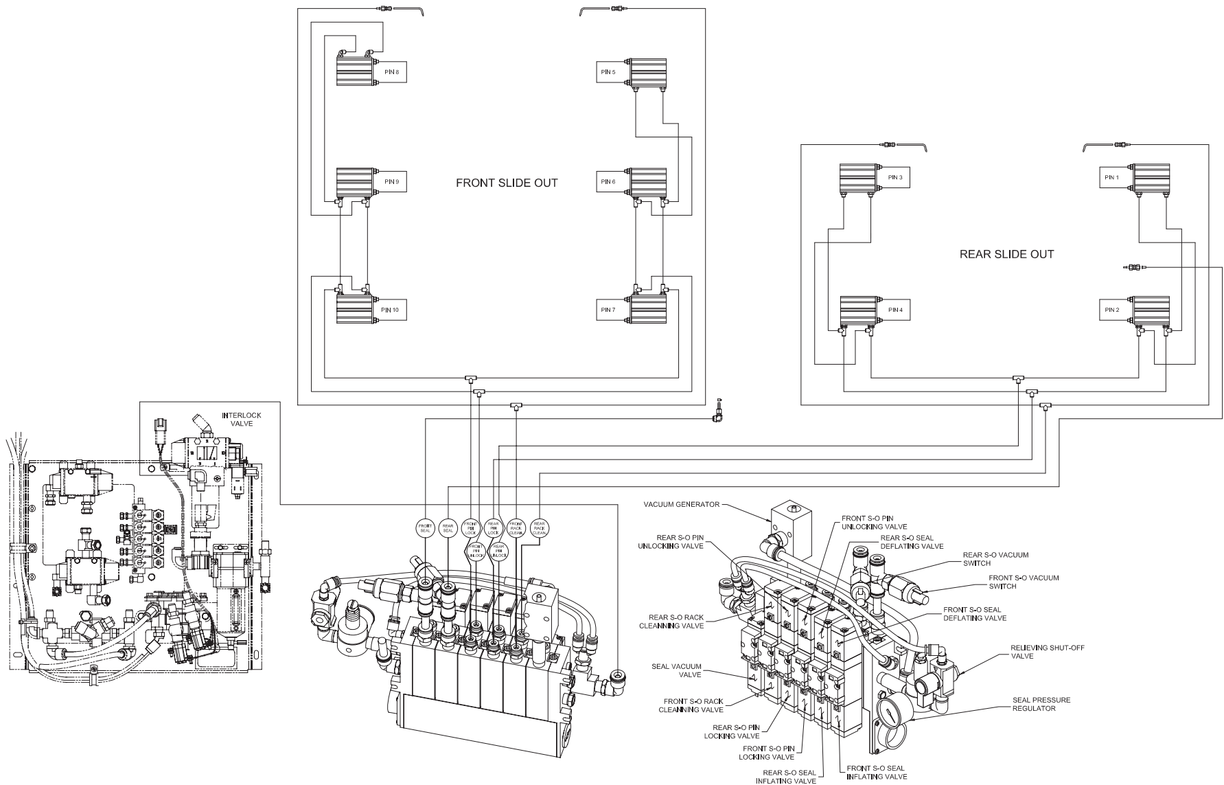
XL2 DOUBLE SLIDE-OUT PNEUMATIC DIAGRAM
